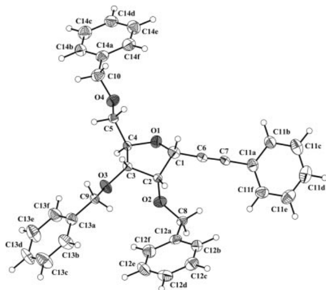
Figure 4. ORTEP diagram of acetylenic 16 \alpha .
