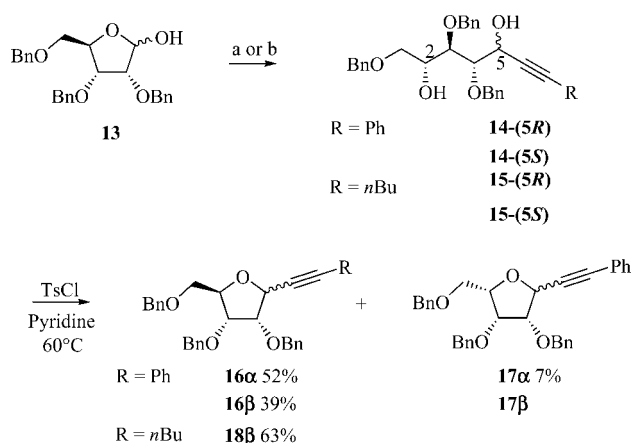
Scheme 2. Reagents and conditions: (a) phenylacetylene (2.2 equiv.), n BuLi (2.0 equiv., 2.4 M in hexanes), THF, -5^{\circ}\text{C} , then 13 (1.0 equiv.) at 10^{\circ}\text{C} and then 2 h at room temp., 87%; (b) hexyne (2.2 equiv.), n BuLi (2.0 equiv., 2.4 M in hexanes), THF, -5^{\circ}\text{C} , then 13 (1.0 equiv.) at 10^{\circ}\text{C} and then 2 h at room temp., 85%.
