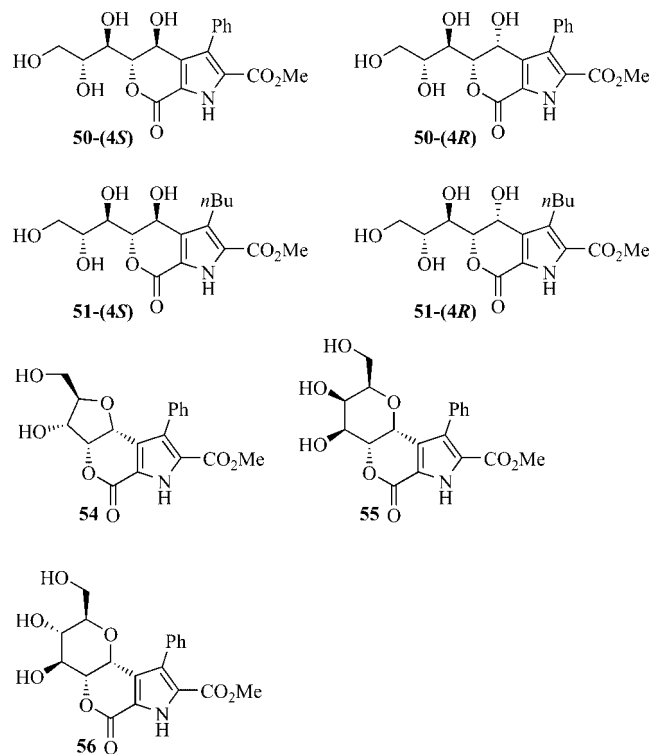
Figure 6. Synthesized polyhydroxy-tetrahydropyrano-pyrroles.
