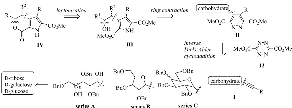
Scheme 1. Retrosynthesis 1.
