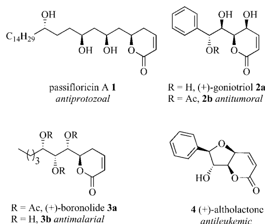
Figure 1. Examples of natural \alpha -pyrones.
