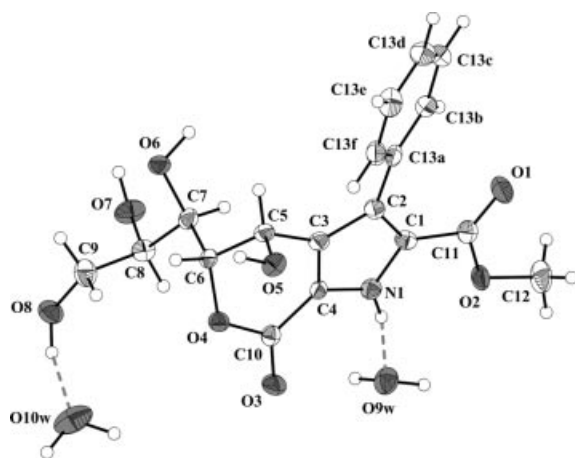
Figure 5. ORTEP diagram of pyrano-pyrone 50-(4S) .
