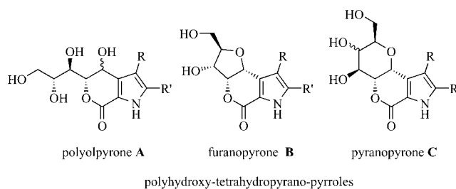
Figure 3. Targeted polyhydroxy-tetrahydropyrano-pyrroles.
