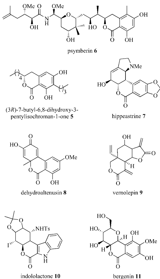
Figure 2. Biologically active compounds presenting an \alpha -pyrone backbone.
